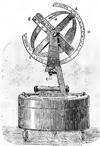
Flechet's Universal Sun-dial.
